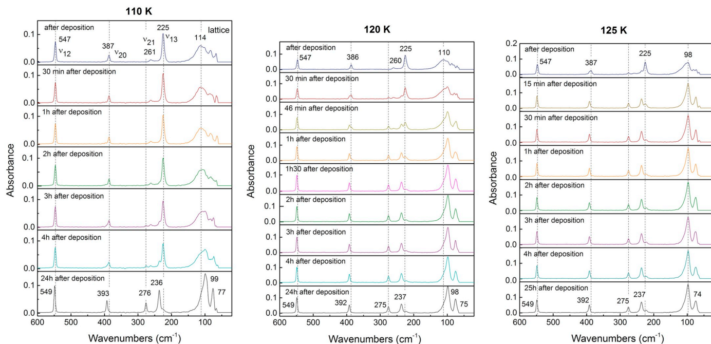
Fig. 6. Temperature and time evolution (up to 25 h after deposition) of far-IR absorbance spectra of C_2H_5CN ice ( 4 \mu m thick film) obtained after deposition of the propionitrile vapors at temperatures of 110 K, 120 K and 125 K. Superimposed in the figures are the vibrational transitions and/or peak frequencies for the observed ice absorption bands.
