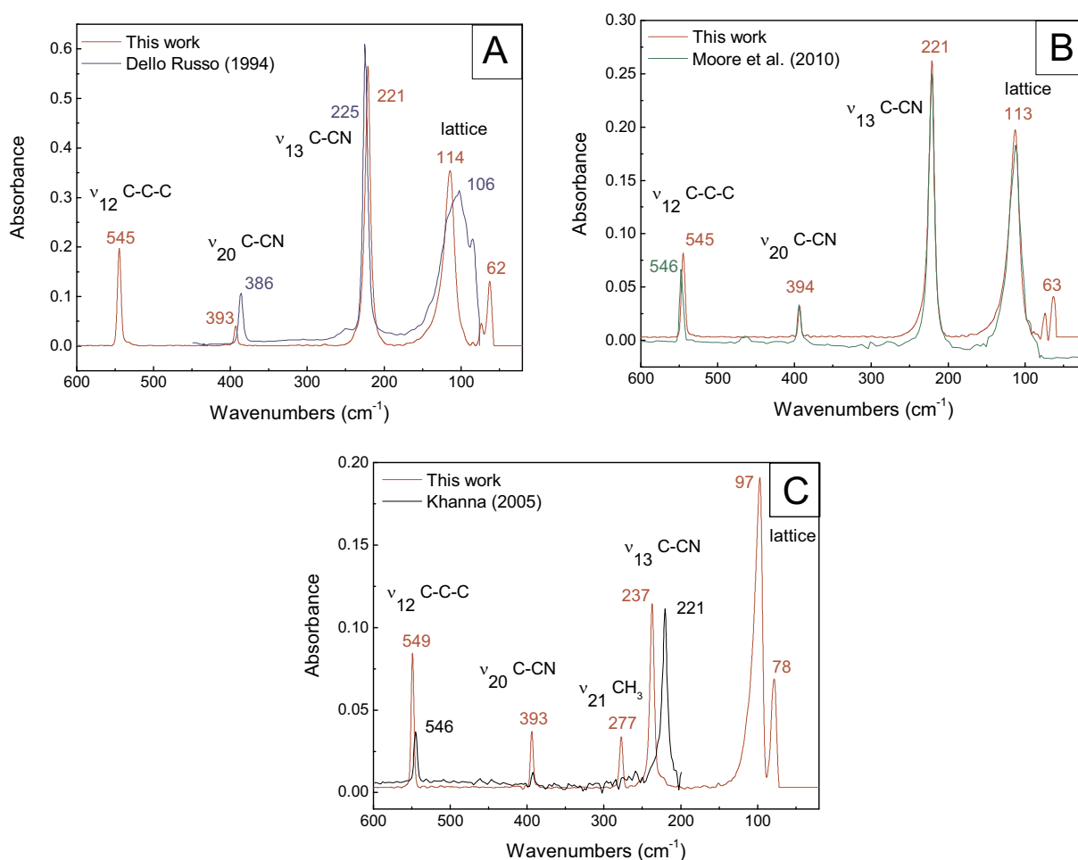
Fig. 4. Comparisons of absorbance spectra of annealed crystalline C_2H_5CN ice between previous experimental studies to those obtained under similar experimental conditions using the SPECTRAL chamber in the SPICE laboratory (current work). (A) The blue curve shows the Dello Russo (1994) absorbance spectrum at 95 K, while the red curve depicts the absorbance spectrum at 95 K from this work, in which C_2H_5CN vapor was deposited at 60 K, annealed at 140 K for 180 min, then cooled to 95 K. (B) The green curve depicts the Moore et al. (2010) absorbance spectrum at 95 K, while the red curve shows the absorbance spectrum at 95 K from this work, in which C_2H_5CN vapor was deposited at 50 K, annealed at 140 K for 90 min, then cooled to 95 K. (C) The black curve shows the Khanna (2005a) absorbance spectrum at 80 K, while the red curve shows the absorbance spectrum at 80 K from this work, in which C_2H_5CN vapor was deposited at 60 K, annealed at 120 K for 240 min, then cooled to 80 K. Superimposed in each figure are the vibrational transitions and peak frequencies for each observed ice absorption band. (For interpretation of the references to colour in this figure legend, the reader is referred to the web version of this article.)
