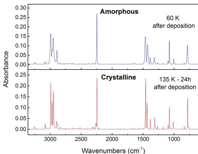
Fig. 13. Mid-IR absorbance spectra from 3350 to 600\text{ cm}^{-1} of amorphous and crystalline \text{C}_2\text{H}_5\text{CN} ice ( 3.95\text{ }\mu\text{m} and 3.85\text{ }\mu\text{m} thick films, respectively) obtained after depositing propionitrile vapors at 60\text{ K} and 135\text{ K} (the latter was held for 24\text{ h} after deposition).
