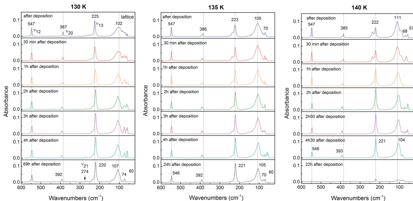
Fig. 8. Temperature and time evolution (up to 69 h after deposition) of far-IR absorbance spectra of crystalline C_2H_5CN ice (4 \mu m thick film) obtained after deposition of the propionitrile vapors at temperatures of 130 K, 135 K and 140 K. Superimposed in the figures are the vibrational transitions and/or peak frequencies for the observed ice absorption bands.
