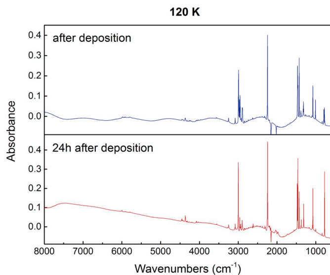
Fig. 7. Mid-IR absorbance raw spectra (channel fringe uncorrected) from 8000 \text{ cm}^{-1} to 600 \text{ cm}^{-1} of C_2H_5CN ice ( 3.84 \mu m thick film) obtained immediately after vapor deposition at 120 K (blue curve on top) and 24 h post-deposition (red curve at the bottom). (For interpretation of the references to colour in this figure legend, the reader is referred to the web version of this article.)
