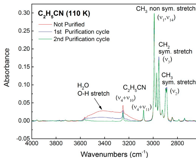
Fig. 2. Mid-IR absorbance spectra of C_2H_5CN ice (vapor deposited at 110 K), indicated by the \nu_2 CH_3 and CH_2 symmetric stretch absorption bands at 2888\text{--}2896\text{ cm}^{-1} and 2953\text{--}2971\text{ cm}^{-1} , respectively; as well as by the \nu_1, \nu_4 CH_3 asymmetric stretch absorption band at 2992\text{ cm}^{-1} and the \nu_4 + \nu_{11} , \nu_4 + \nu_{10} vibration modes at 3079\text{ cm}^{-1} and 3249\text{ cm}^{-1} , respectively. The three colour-coded curves depict various degrees of H_2O contamination (shown by the broad O–H stretch absorption band between 3200 and 3600\text{ cm}^{-1} ) in the C_2H_5CN sample, following numerous freeze-pump-thaw cycles under vacuum using a -116^\circ\text{C} C_2H_5OH/LN_2 cold bath. The red curve shows a 3.6\text{ }\mu\text{m} thick film of C_2H_5CN ice for the unpurified C_2H_5CN sample, which contains a significant amount of H_2O . The blue curve shows the ice film of the same C_2H_5CN sample (with the same thickness as previously) following nine freeze-pump-thaw cycles (1st purification cycle), with a reduced amount of H_2O visible in the spectrum. The green curve of C_2H_5CN ice film shows the final purified C_2H_5CN ice spectrum obtained after four additional freeze-pump-thaw cycles (2nd purification cycle), giving a total of thirteen freeze-pump-thaw cycles, with the amount of H_2O contamination now below the FTIR spectrometer detection limit. (For interpretation of the references to colour in this figure legend, the reader is referred to the web version of this article.)
