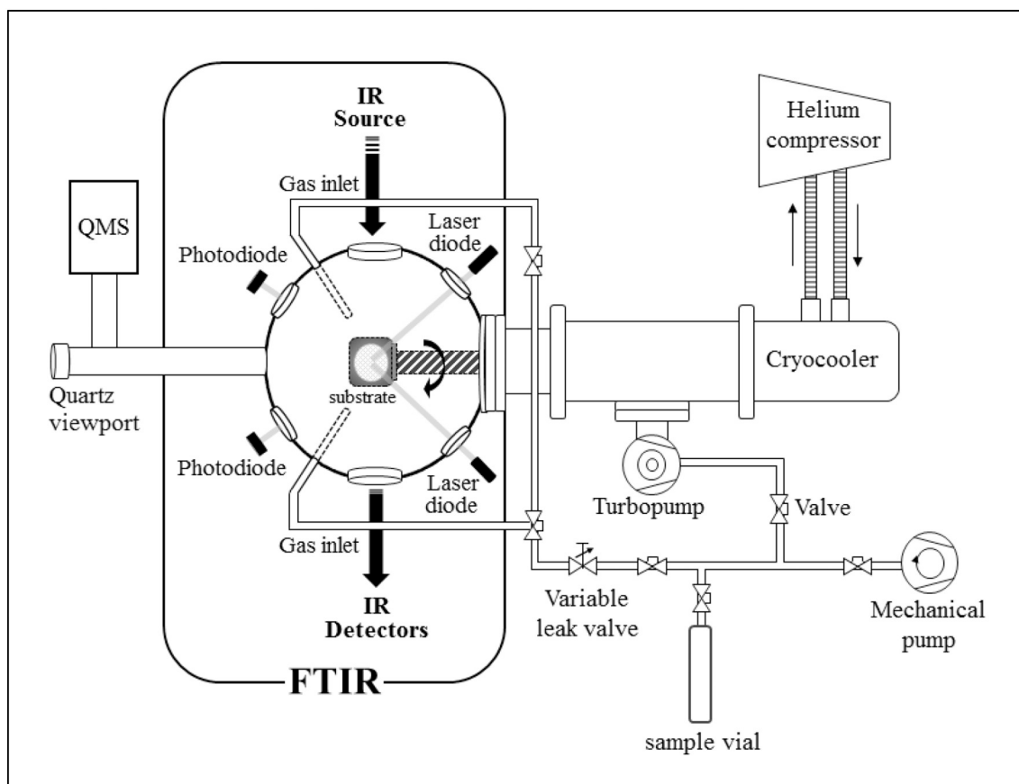
Fig. 3. Schematic illustration of the experimental setup used for the C_2H_5CN ice experiments in the SPECTRAL ice chamber (modified from Anderson et al., 2018a). Vapor deposition of C_2H_5CN onto a cold diamond substrate (30 K – 160 K) forms a thin ice film that is monitored in situ by IR transmission spectroscopy from 50\text{ cm}^{-1} to 11,700\text{ cm}^{-1} ( 200\text{--}0.85\text{ }\mu\text{m} ) through a FTIR spectrometer. Double laser interferometry is used to determine the thickness of the ice films.
