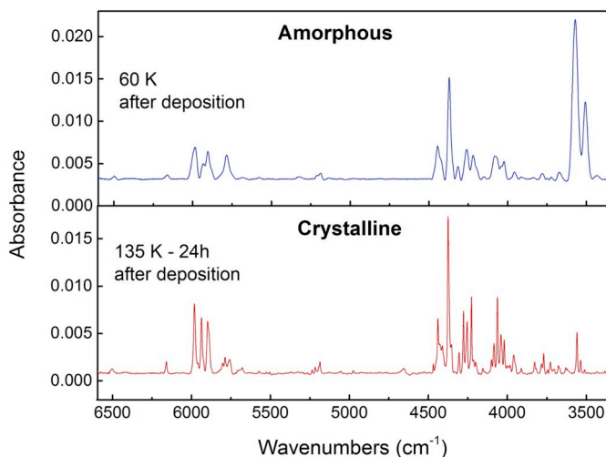
Fig. 14. Mid-IR absorbance spectra from 6600 to 3350\text{ cm}^{-1} of amorphous and crystalline \text{C}_2\text{H}_5\text{CN} ice ( 3.95\text{ }\mu\text{m} and 3.85\text{ }\mu\text{m} thick films, respectively) obtained after depositing propionitrile vapors at 60\text{ K} and 135\text{ K} (the latter was held for 24\text{ h} after deposition).
