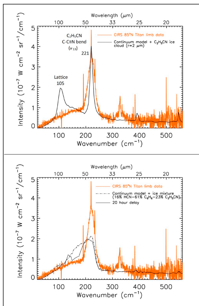
Fig. 15. Cassini CIRS far-IR limb integration spectra of Titan recorded at a tangent height of 136 km in March 2005 at 85^\circ N (orange curves). Twelve spectra are contained in the limb-integration averages. The black curves are synthetic spectra of our radiative transfer continuum model coupled with Mie scattering calculations for pure C_2H_5CN ice (upper panel) and a ternary ice mixture containing 16% HCN, 23% C_2H_5CN , and 61% C_6H_6 (lower panel). The optical constants were derived from our laboratory absorbance spectra of crystalline C_2H_5CN ice (24 h after vapor deposition at 135 K; upper black curve) and the ternary HCN- C_2H_5CN - C_6H_6 ice (mixed vapors deposited at 110 K; lower black curves), following the method described in Anderson et al. (2018a). The dash-dot black curve in the lower panel represents the ternary ice directly after vapor deposition, while the solid black curve shows the ternary ice after a 20 h delay. Superimposed in the upper panel are the vibrational transitions and peak frequencies for the observed C_2H_5CN ice absorption bands.
