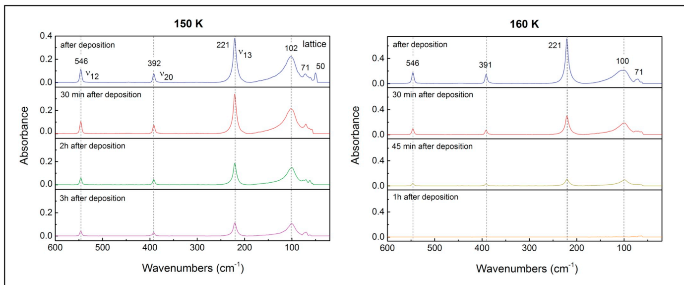
Fig. 9. Temperature and time evolution (up to 3 h after deposition) of far-IR absorbance spectra of crystalline C_2H_5CN ice obtained just after deposition of the propionitrile vapors at temperatures of 150 K and 160 K. For these temperatures, C_2H_5CN sublimates rapidly so thicker ice films of 15 \mu m (at 150 K) and 7.5 \mu m (at 160 K) were grown on the diamond substrate. Tentatively, a thick ice film \geq 15 \mu m was grown and analyzed at 160 K in order to leave the sample longer than 1 h after deposition before the ice sublimated. However, several absorption bands of propionitrile appeared very saturated with such a thick sample. Superimposed in the figures are the vibrational transitions and/or peak frequencies for the observed ice absorption bands.
