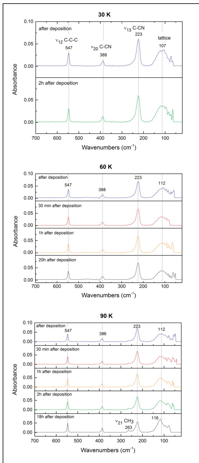
Fig. 5. Temperature and time evolution (up to 20 h after deposition) of far-IR absorbance spectra of amorphous C_2H_5CN ice ( 4 \mu m thick film) obtained after deposition of the propionitrile vapors at temperatures of 30 K, 60 K and 90 K. Superimposed in the figures are the vibrational transitions and/or peak frequencies for the observed ice absorption bands.
