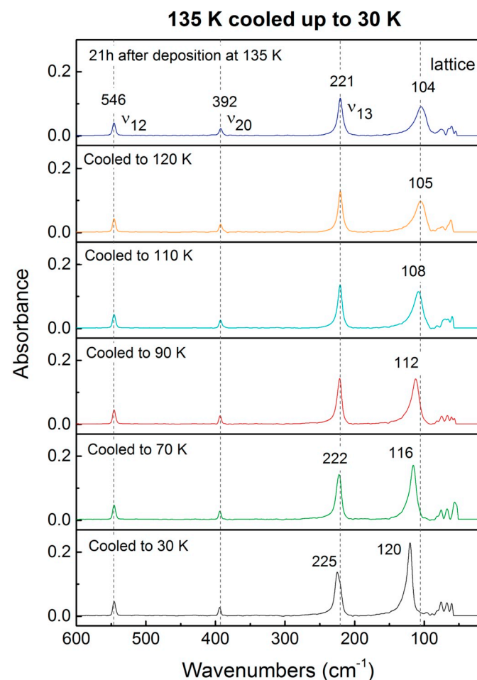
Fig. 11. Far-IR absorbance spectra of crystalline \text{C}_2\text{H}_5\text{CN} ice ( 3.77 \mu\text{m} thick film) deposited at 135 K and held at this temperature for 21 h after deposition, then cooled to 120 K, 110 K, 90 K, 70 K, and 30 K. Superimposed in the figures are the vibrational transitions and/or peak frequencies for the observed ice absorption bands.
