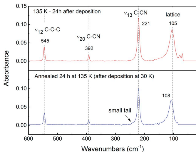
Fig. 10. Far-IR absorbance spectra of crystalline \text{C}_2\text{H}_5\text{CN} ice deposited at 135 K and held at 135 K for 24 h post-deposition (red curve on top) compared to \text{C}_2\text{H}_5\text{CN} ice deposited at 30 K and then annealed at 135 K for 24 h (blue curve at the bottom). For both samples, the ice film thickness was \sim 4 \mu\text{m} . Superimposed in the figure are the vibrational transitions and peak frequencies for the observed ice absorption bands. (For interpretation of the references to colour in this figure legend, the reader is referred to the web version of this article.)
