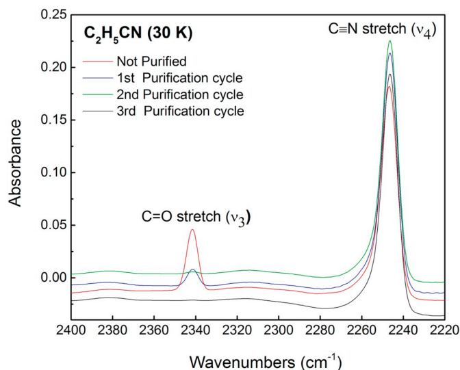
Fig. 1. Mid-IR absorbance spectra of amorphous C_2H_5CN ice (vapor deposited at 30 K), indicated by the \nu_4 C\equiv N stretch absorption band at 2246\text{ cm}^{-1} . The four colour-coded curves depict various degrees of CO_2 contamination (shown by the \nu_3 C=O stretch absorption band at 2342\text{ cm}^{-1} ) in the C_2H_5CN sample, following numerous freeze-pump-thaw cycles under vacuum using a -116^\circ\text{C} C_2H_5OH/LN_2 cold bath. The red curve shows a 4.2\text{ }\mu\text{m} thick film of C_2H_5CN ice for the unpurified C_2H_5CN sample, which contains a significant amount of CO_2 . The blue curve shows the ice film of the same C_2H_5CN sample (with the same thickness as previously) following five freeze-pump-thaw cycles (1st purification cycle), with a reduced amount of CO_2 visible in the spectrum. The green curve of C_2H_5CN ice film is obtained after four additional freeze-pump-thaw cycles (2nd purification cycle), with CO_2 now visible as a trace contaminant in the C_2H_5CN ice sample. The black curve shows the final purified C_2H_5CN ice spectrum, after a total of thirteen freeze-pump-thaw cycles (3rd purification cycle), with the amount of CO_2 contamination now below the FTIR spectrometer detection limit. (For interpretation of the references to colour in this figure legend, the reader is referred to the web version of this article.)
