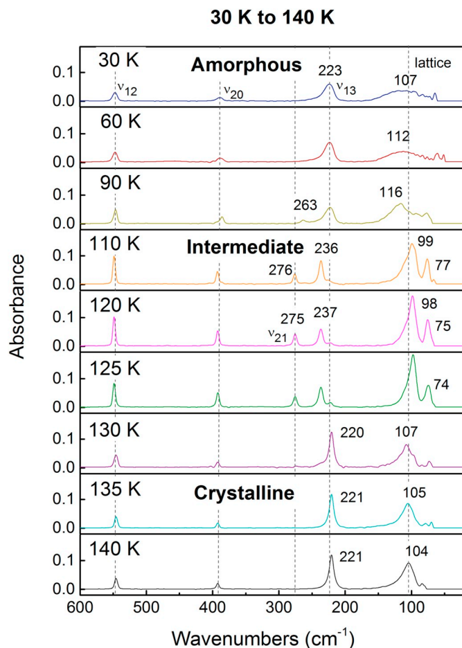
Fig. 12. Far-IR absorbance spectra of amorphous to crystalline C 2 H 5 CN ice ( \sim 4 \mu\text{m} thick film) obtained after depositing propionitrile vapors at temperatures from 30 K to 140 K and held several hours after deposition until no further spectral changes were observed. Superimposed in the figures are the peak frequencies for the observed ice absorption bands that are temperature-dependent.
