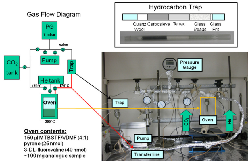
Fig. 2. Flow diagram and picture of the experimental setup used in this study to extract organic compounds from Mars analog materials and concentrate the MTBSTFA derivatization products on a SAM-like hydrocarbon trap for GCMS analyses (commercial pyrolysis GCMS instrument not shown).
