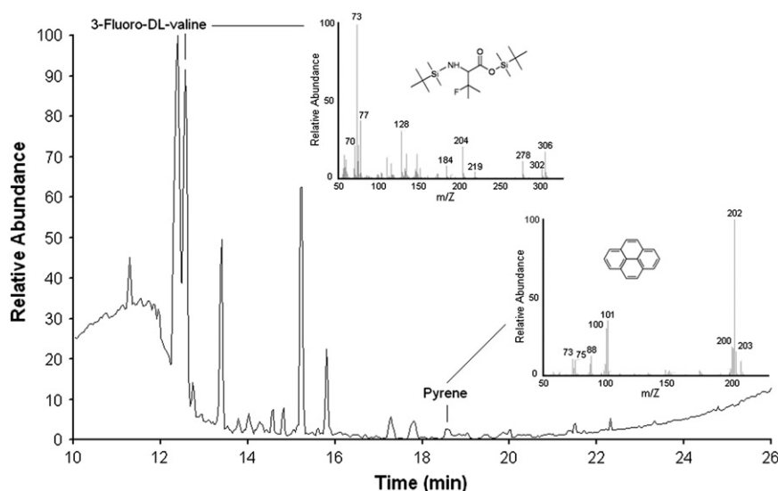
Fig. 5. GCMS analysis of the hydrocarbon trap after derivatization of the fused silica procedural blank (Quartz-01) with 150 \mu\text{L} of MTBSTFA-DMF at 300 ^{\circ}\text{C} for 3 min. The others peaks are also present in the blank (MTBSTFA/DMF only, no 3-FV) and are polysiloxanes or reaction products from the hydrocarbon trap. Experimental conditions: the initial temperature of the column was kept at 140 ^{\circ}\text{C} . After 10 min at 140 ^{\circ}\text{C} , the GC oven was ramped to 300 ^{\circ}\text{C} at a rate of 10 ^{\circ}\text{C}/\text{min} . The final temperature of the column was maintained at 300 ^{\circ}\text{C} for 10 min. A mass spectrometer solvent delay of 10 min from the time of GC injection was included. Top and right: mass spectrum of 3-FV derivative and pyrene extracted from sample.
