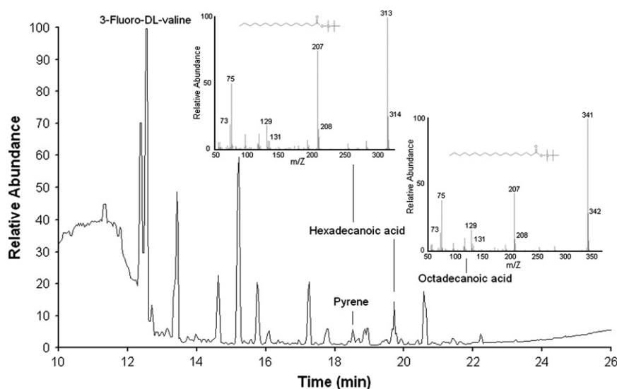
Fig. 6. GCMS chromatograms of the hydrocarbon trap after "one-pot" extraction and derivatization of the Atacama Desert surface (Atacama-01) soil at 300 ^{\circ}\text{C} . Top and right: mass fragmentation spectra pattern of octadecanoic acid and hexadecanoic acid derivatives extracted from sample. Experimental conditions: the initial temperature of the column was kept at 140 ^{\circ}\text{C} . After 10 min at 140 ^{\circ}\text{C} , the GC oven was ramped to 300 ^{\circ}\text{C} at a rate of 10 ^{\circ}\text{C}/\text{min} . The final temperature of the column was maintained at 300 ^{\circ}\text{C} for 10 min. A mass spectrometer solvent delay of 10 min from the time of GC injection was included. Fragmentation patterns for MTBSTFA/DMF, 3-FV and pyrene is not shown.
